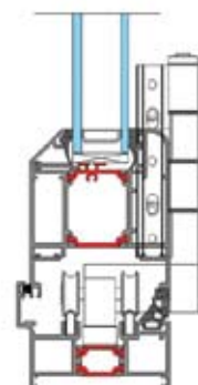
Cill Detail
