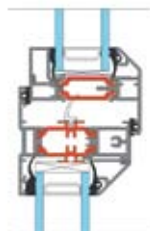
Vent / Transom Detail
