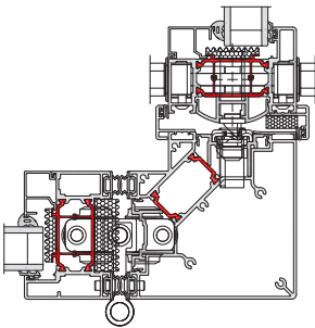
F82 PLUS FLOATING CORNER POST
